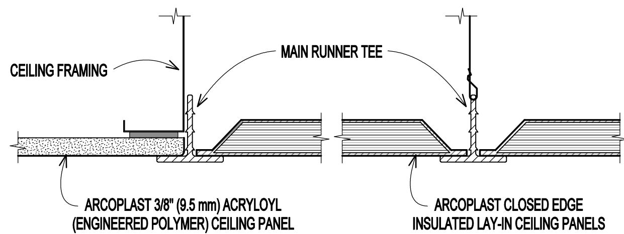
PARTIAL CEILING SECTION SCALE: 6" = 1'-0"
