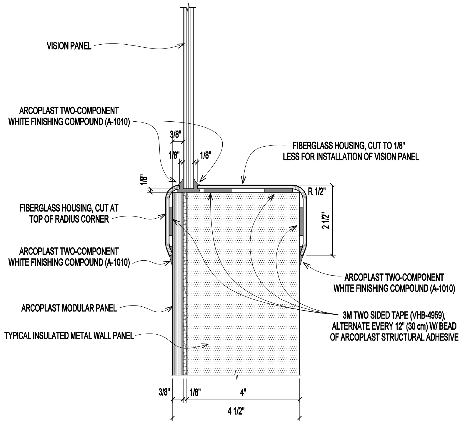
WINDOW FRAME DETAILS SCALE: 6" (1:2)
