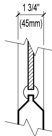
SECTION - A
