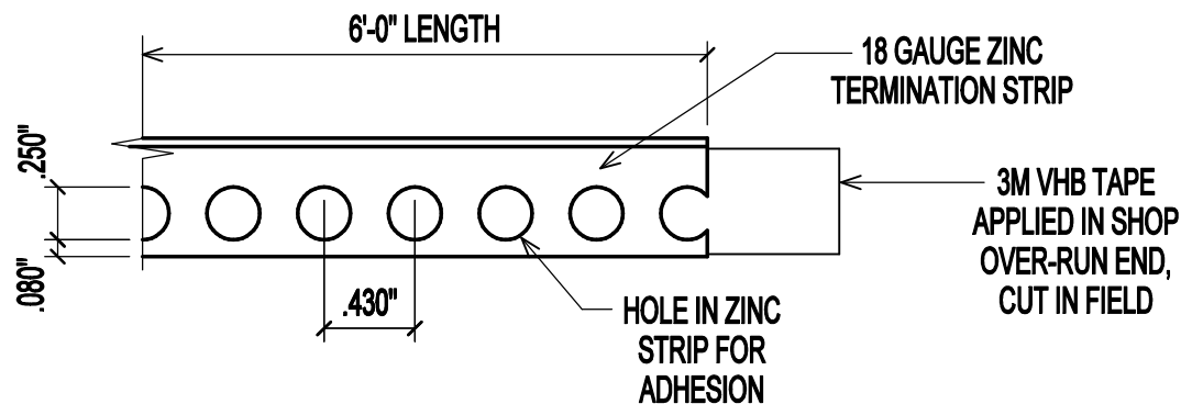
PARTIAL FRONT VIEW FULL SCALE
