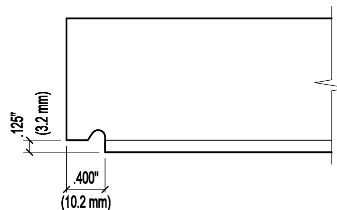
ENLARGED COPE DETAIL - #TR-6011 - TYPICAL EACH END FULL SCALE
