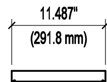
TR-35 - 1 FOOT CROSS RAIL - #TR-6011 SCALE: 1"=1'-0" (1:12)
